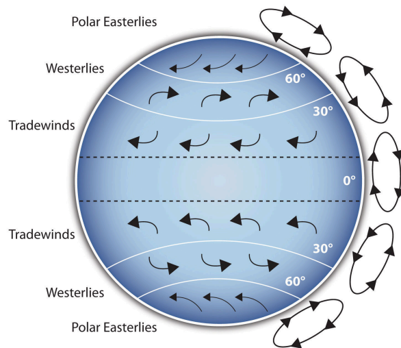
Figure 12.1 – Coriolis Effect
